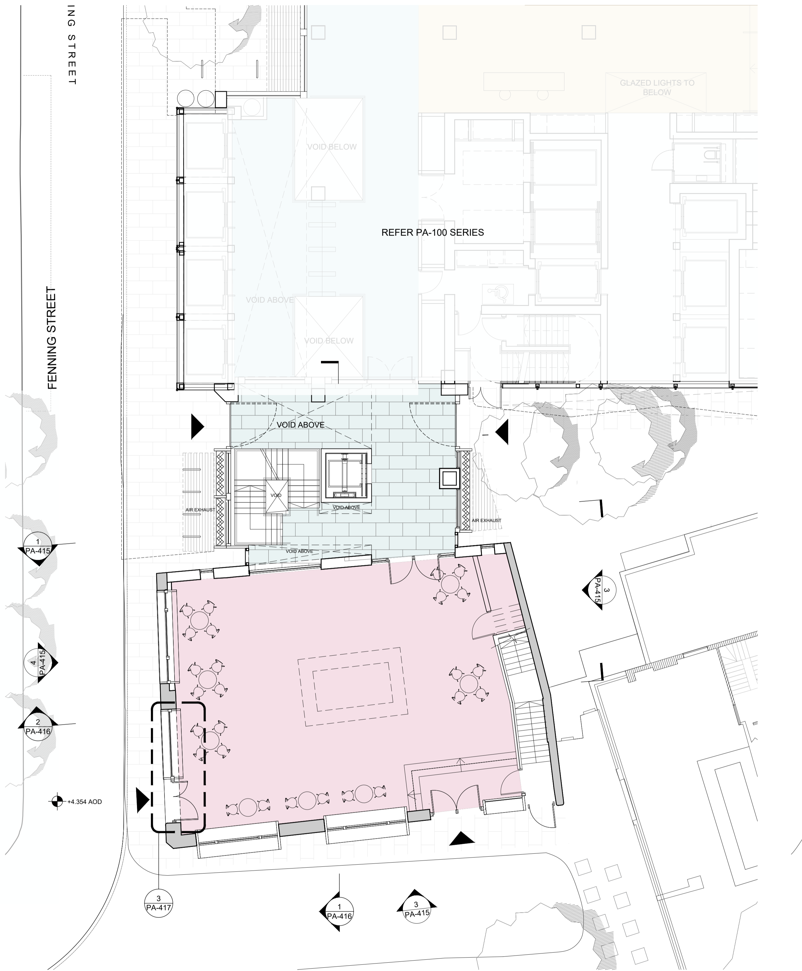
1 PLAN - WAREHOUSE LEVEL 0 SCALE: 1:100
