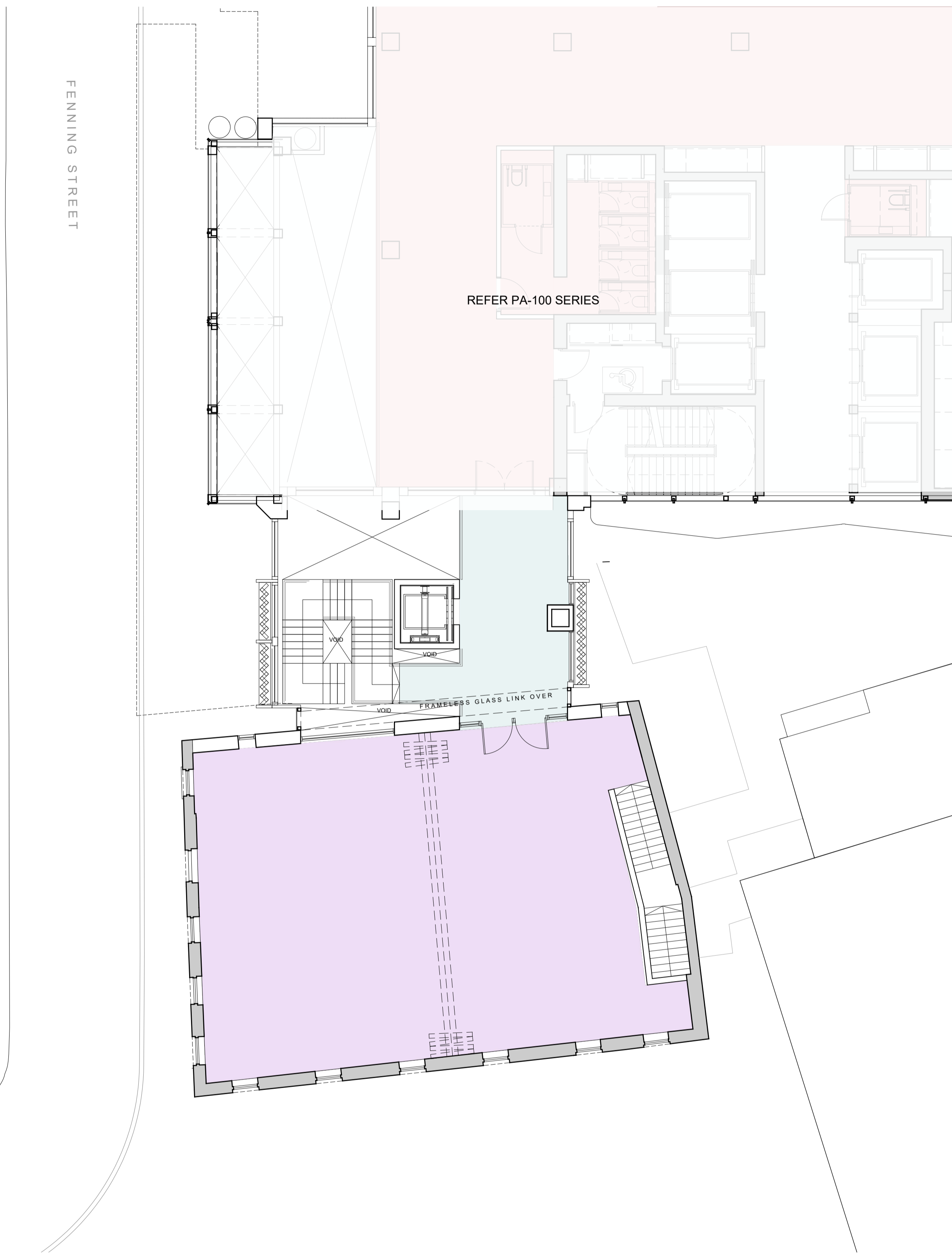
2 PLAN - WAREHOUSE LEVEL 1 SCALE: 1:100
