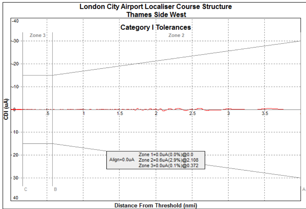
Figure 3: Localiser runway 09 course structure
