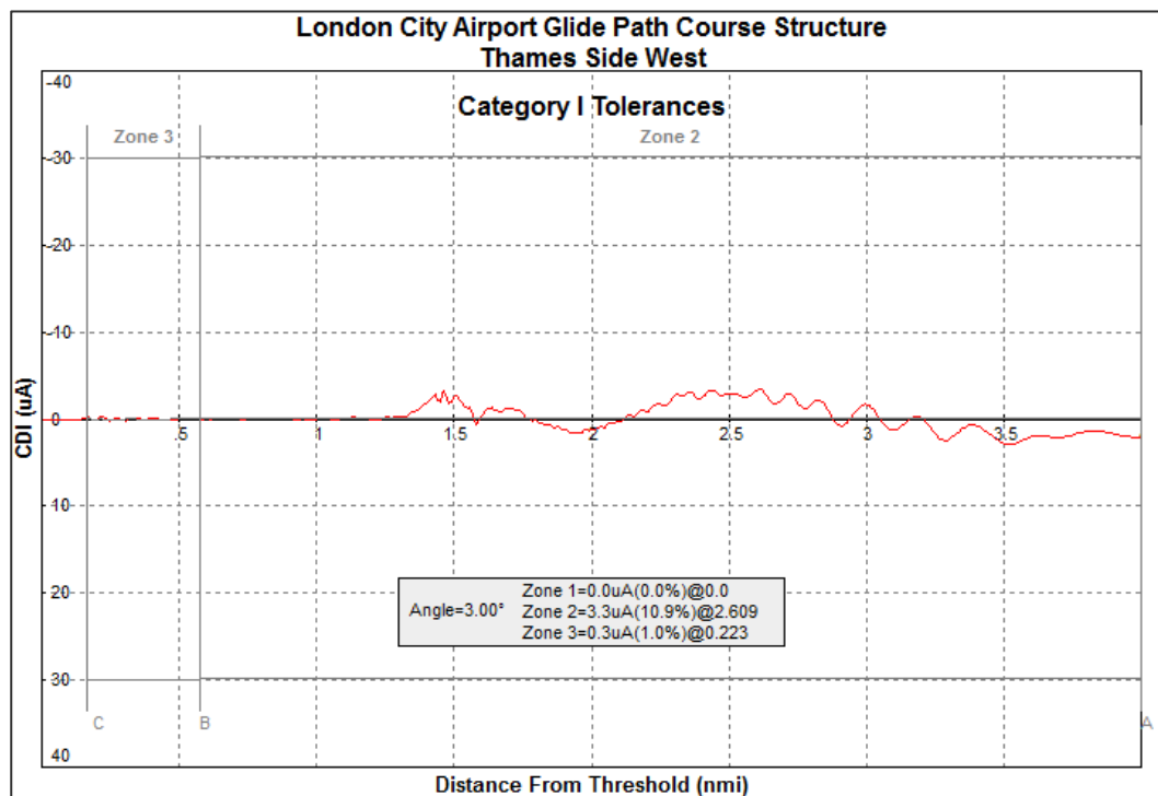
Figure 5: Glide path runway 09 course structure
