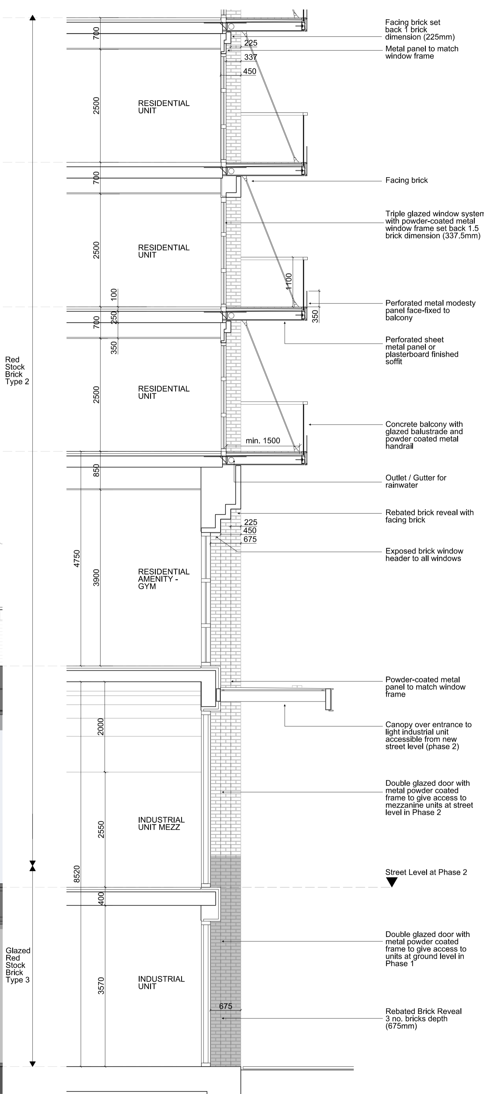
02 TYPICAL BAY 01 - SECTION 1:50
