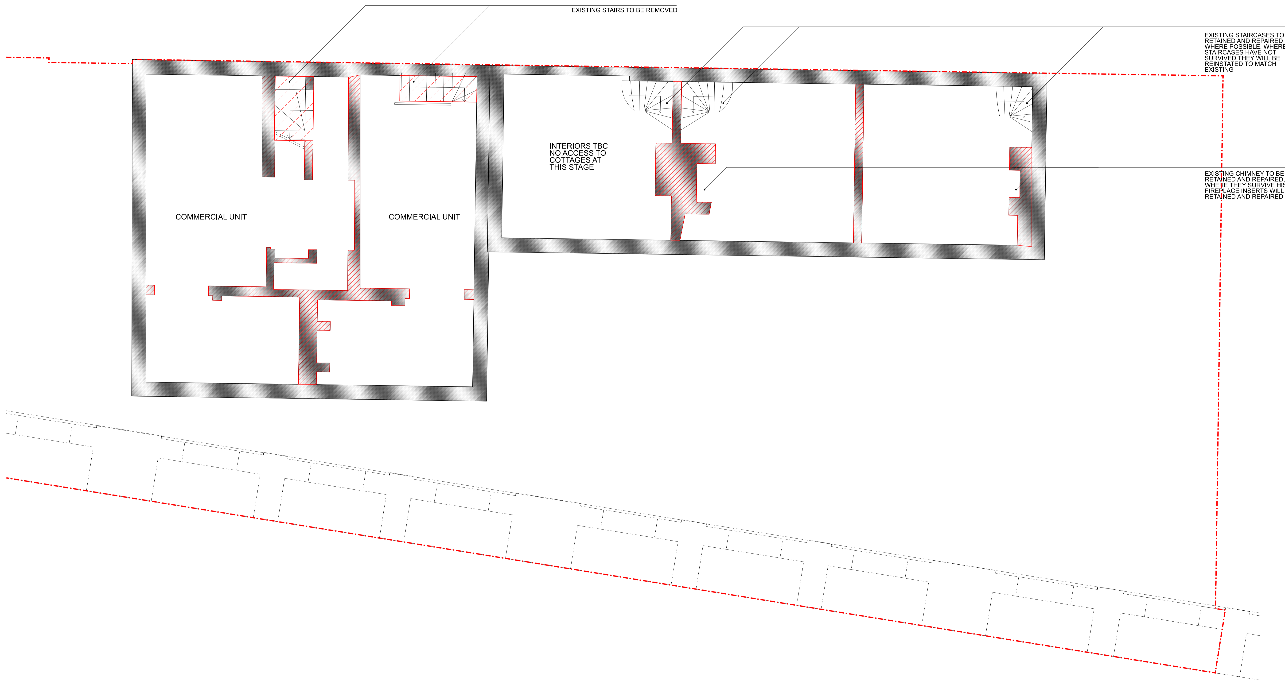
1 1:50 @ A1 / 1:100 @ A3 EXISTING BASEMENT PLAN
