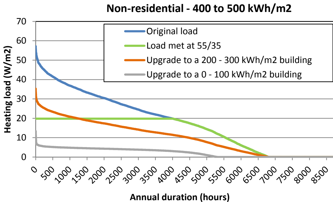
Figure 3-10 – Impact on load duration curve of upgrading the fabric of a poor quality building by one rating (orange line) and by two ratings (grey line) – non-residential
