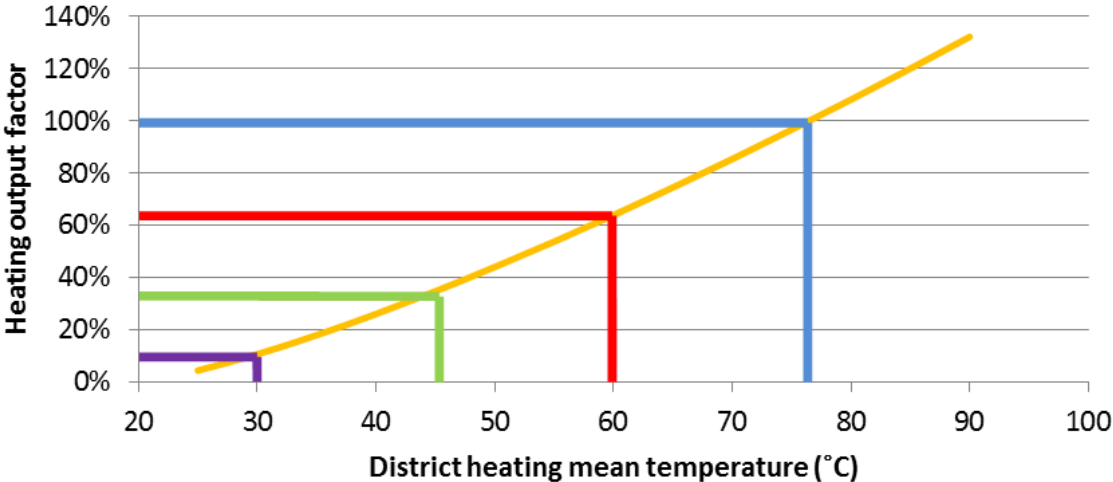
Figure 3-3 – District heating mean temperature vs heat output factor for radiator system peak load. The blue line highlights the mean temperature and corresponding output factor for flow/return temperatures of 82/71°C; the red line highlights the equivalent for 70/50°C; the green line for 50/35°C; and the purple line for 40/20°C. The colours correspond to those used in figures 3-5 to 3-8 for the same flow and return temperatures
