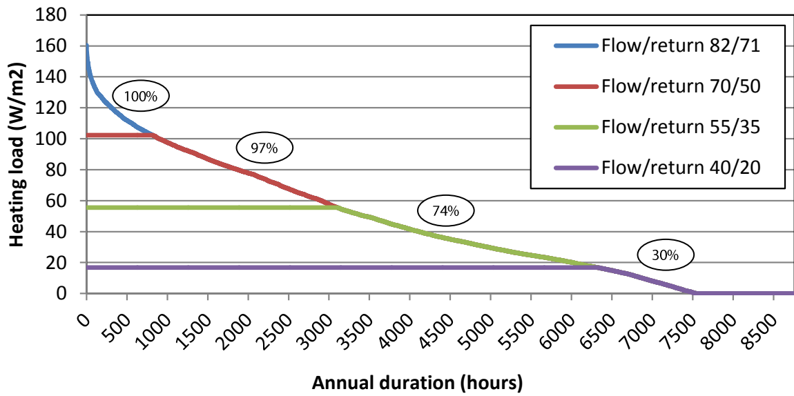
Figure 3-6 – Annual heat demand percentage met by heat supply temperatures – residential low build quality
