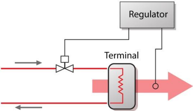
Figure 4-1 – Principle of two port control for terminal devices
