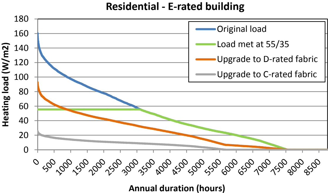
Figure 3-9 – Impact on load duration curve of upgrading the fabric of a poor quality building by one rating (orange line) and by two ratings (grey line) - residential
