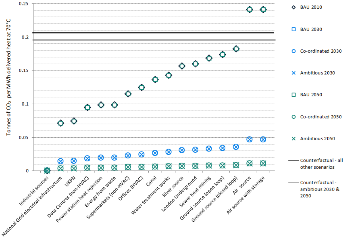
Figure 2-4 – Carbon intensity of heat supply sources by scenario
