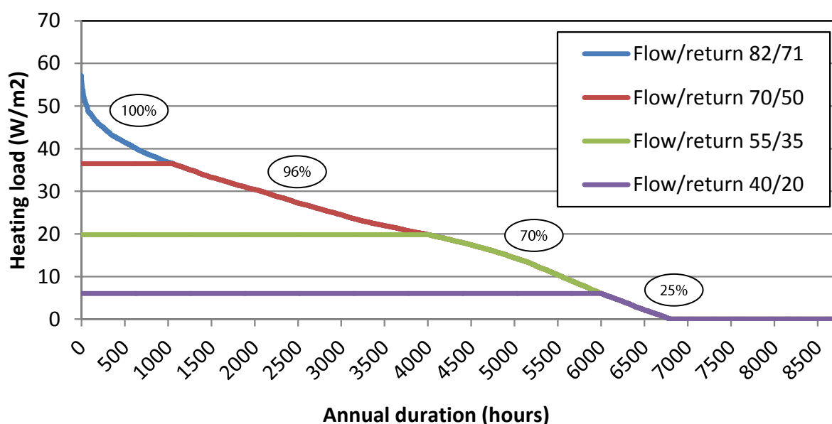
Figure 3-8 – Annual heat demand percentage met by heat supply temperatures –non-residential low build quality
