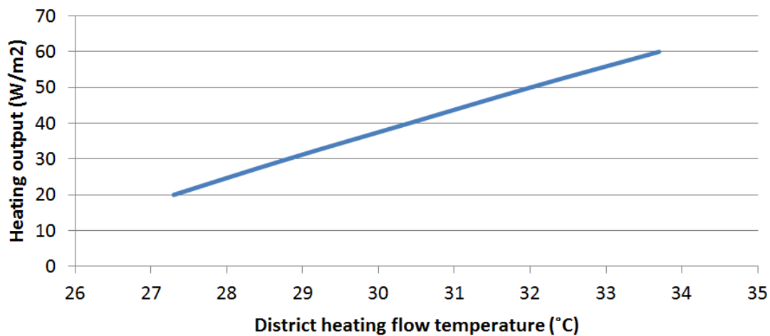
Figure 3-4 – Heat output vs flow temperature for a typical underfloor heating system with tiled finish 17
