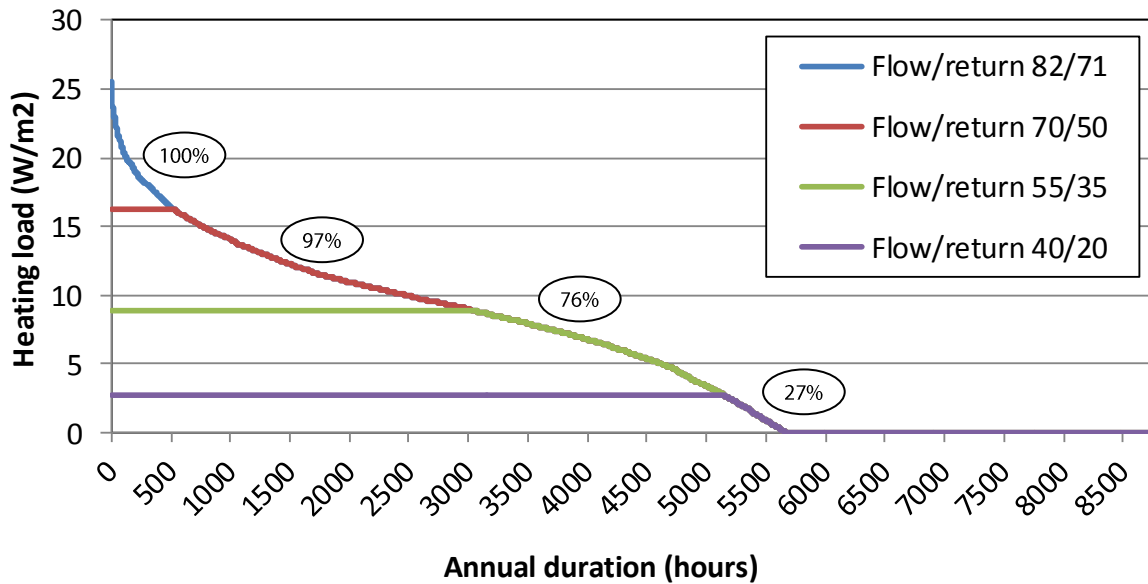
Figure 3-5 – Annual heat demand percentage met by heat supply temperatures – residential high build quality
