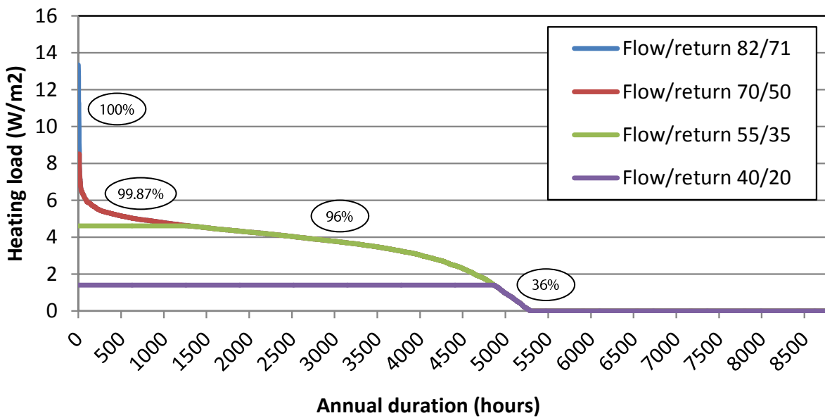
Figure 3-7 – Annual heat demand percentage met by heat supply temperatures – non-residential high build quality
