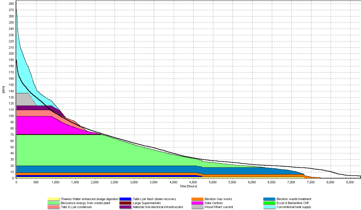
Figure 6-8 – Duration curve for pilot study heat supply
