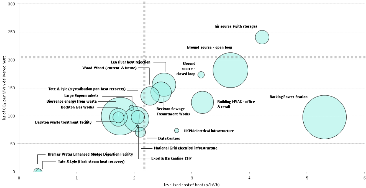
Figure 6-5 – Carbon intensity v levelised cost of secondary heat sources within the Pilot Study area (BAU 2010)
