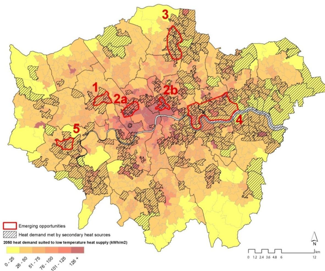
Figure 6-1 – Emerging opportunities for low temperature heat networks
