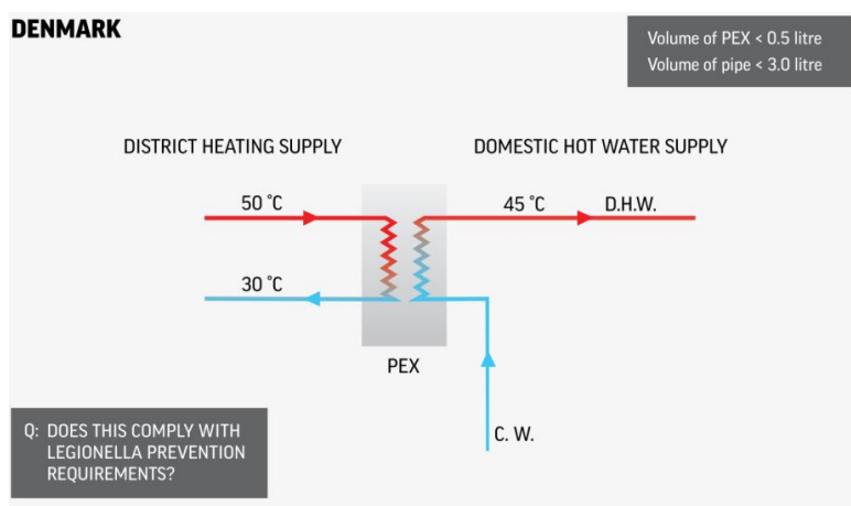
Figure 3-2 – Danish heat network temperatures in new buildings for domestic hot water supply
