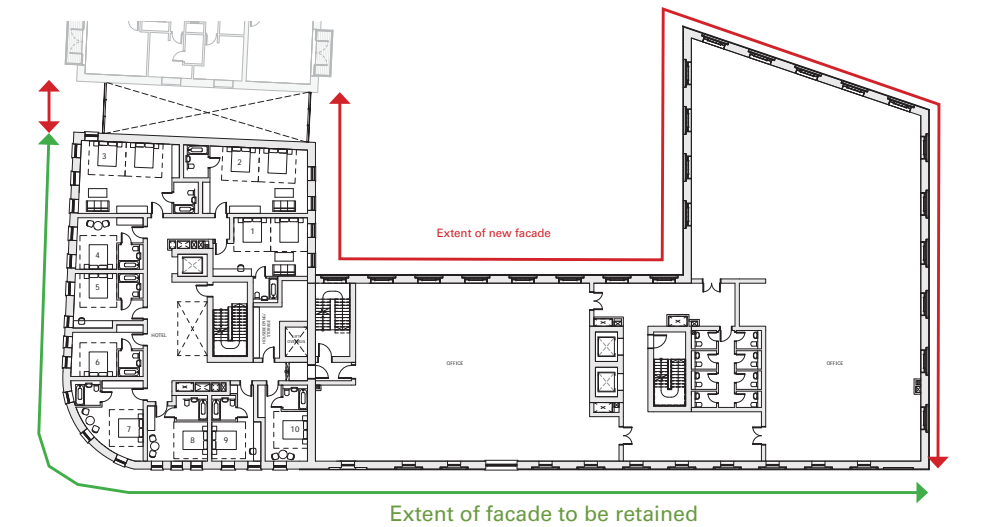
ORIGINAL PROPOSAL: BUILDING 5 FIRST FLOOR PLAN
