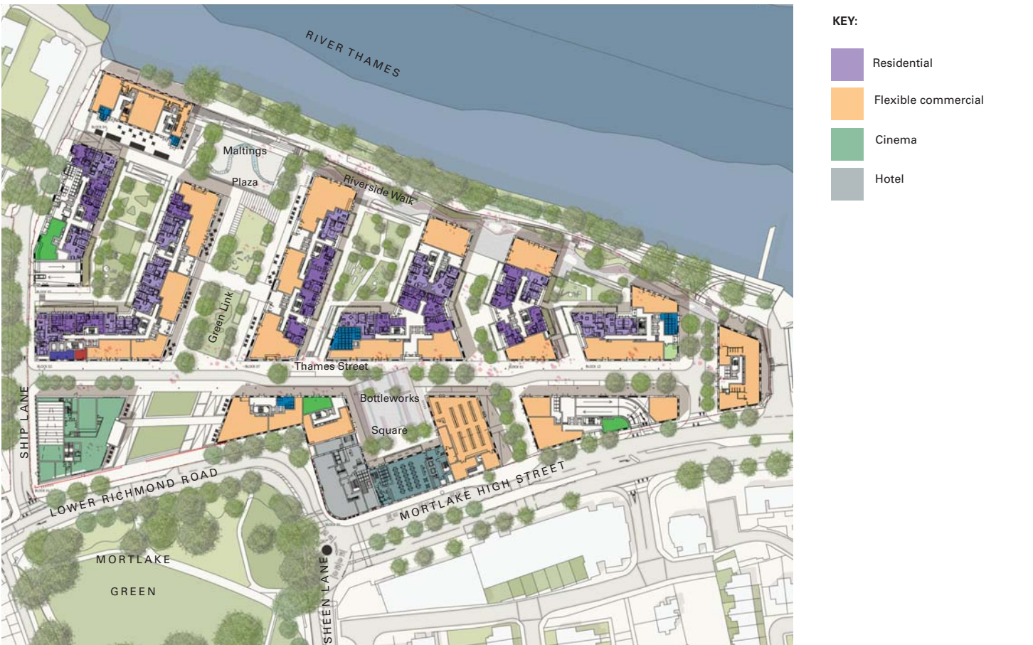
ORIGINAL PROPOSAL: GROUND FLOOR LEVEL MASTERPLAN
