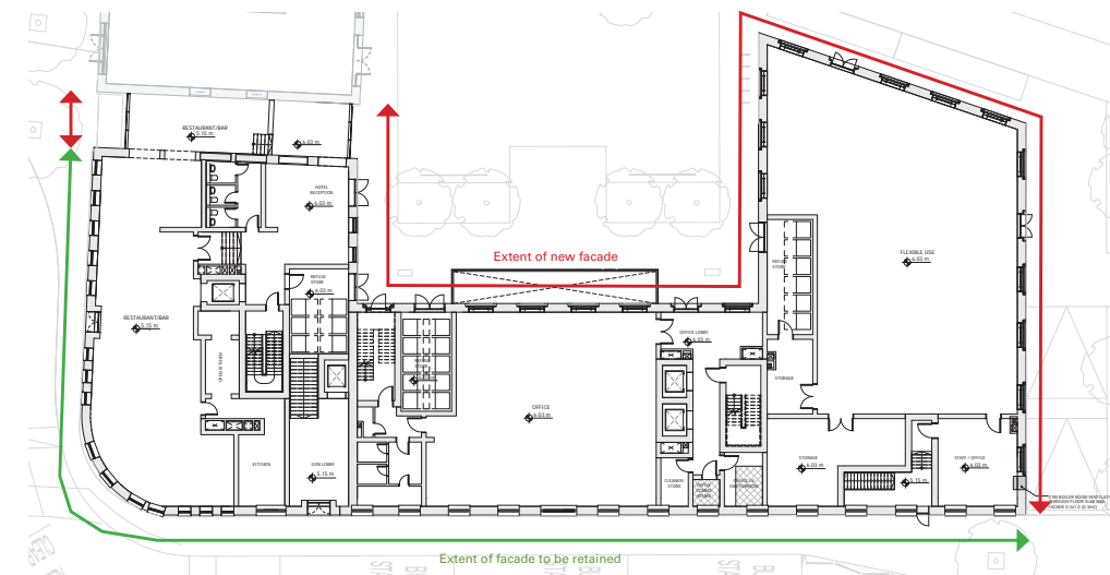
ORIGINAL PROPOSAL: BUILDING 5 GROUND FLOOR PLAN
