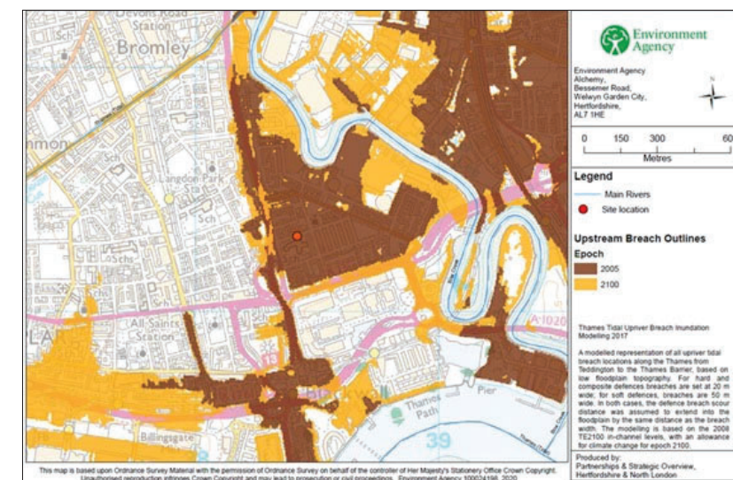
Figure 9 – Modelled Flood Extent – Breach. Tidal Upriver Breach Inundation Modelling Study 2017
