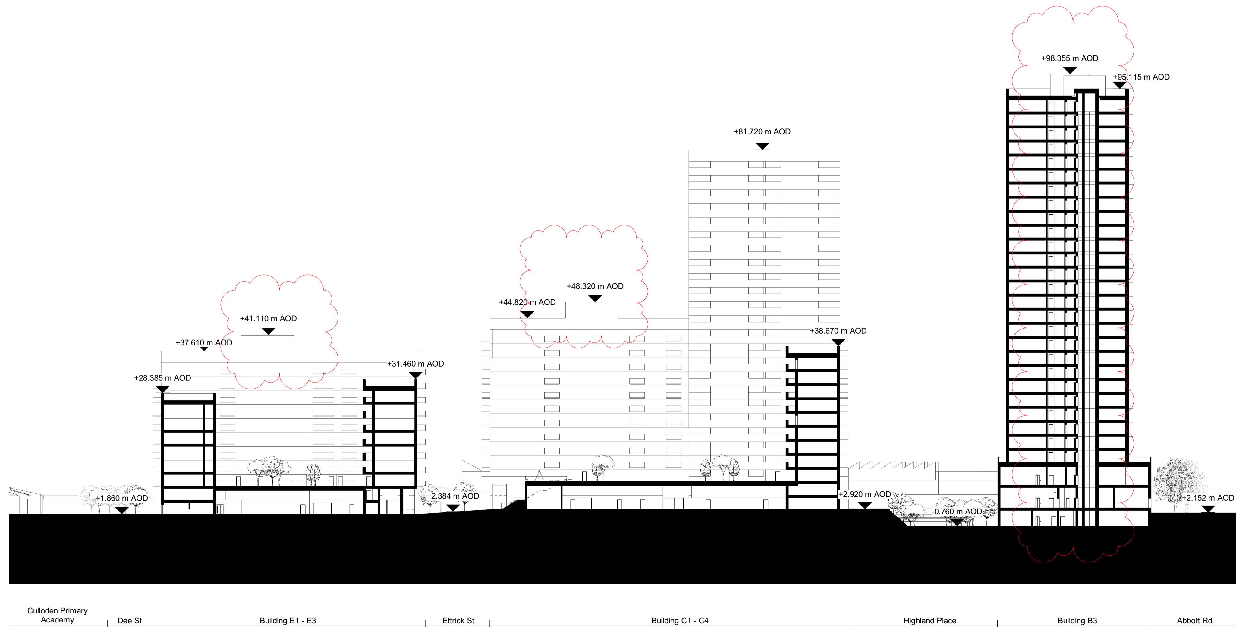
02 Section
