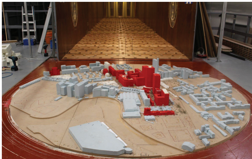
Figure 17: Proposed Development (Illustrative Scheme) and Phase A with Existing Surrounding Buildings, Proposed Landscaping and Wind Mitigation Measures (Configuration 5, Board 1) – View in the Wind Tunnel (from the north)
