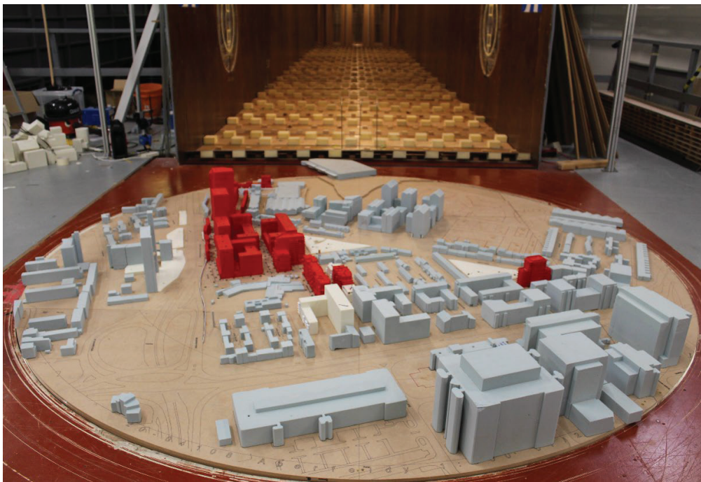
Figure 13: Proposed Development (Outline Proposals plus Detailed Proposals) with Existing Surrounding Buildings (Configuration 3, Board 2) – View in the Wind Tunnel (from the south)
