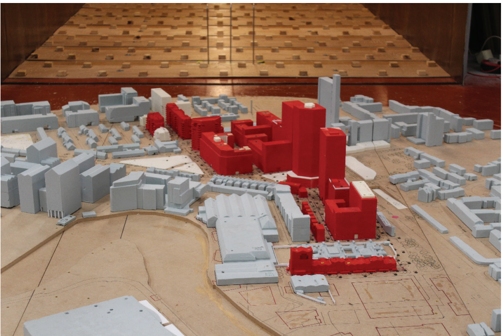
Figure 16: Proposed Development (Illustrative Scheme) and Phase A with Existing Surrounding Buildings (Configuration 4, Board 1) – View in the Wind Tunnel (from the north)
