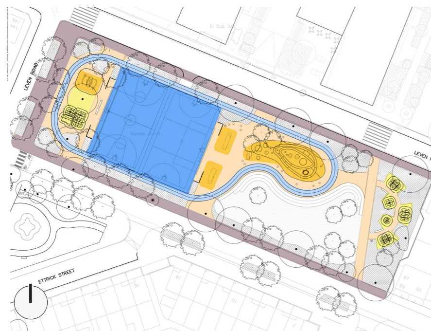
Surface Finishes Plan - Leven Park
