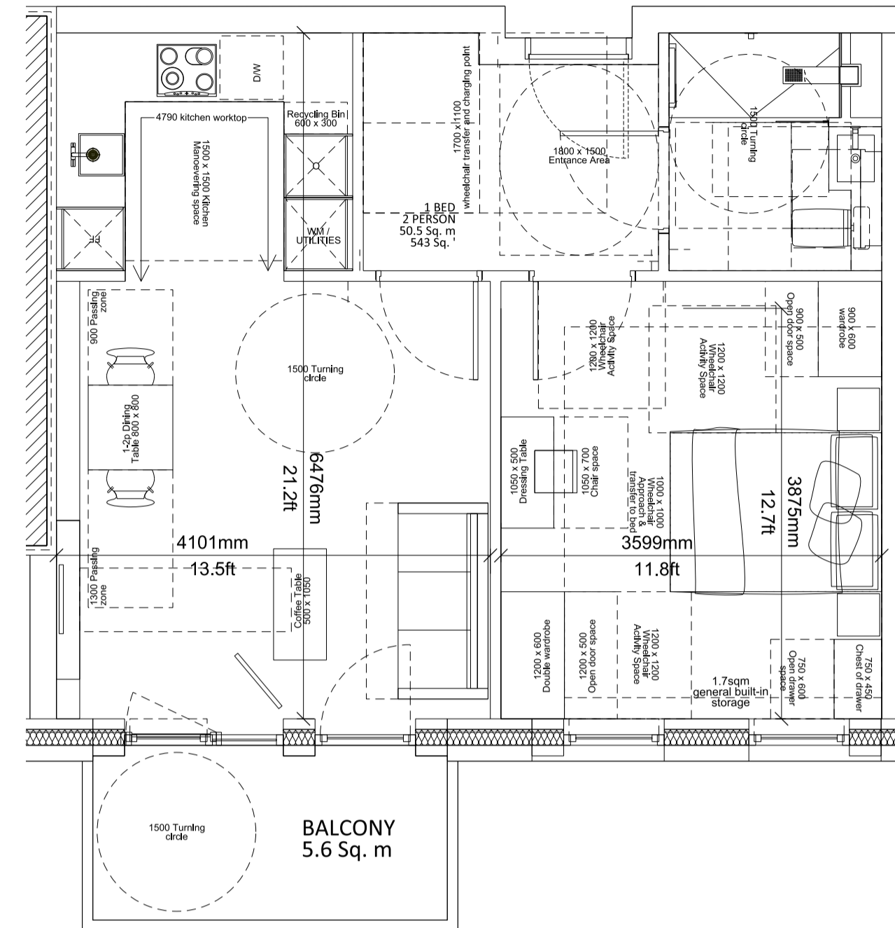
02 1 Bed Apartment M4(3)(2)(a)
