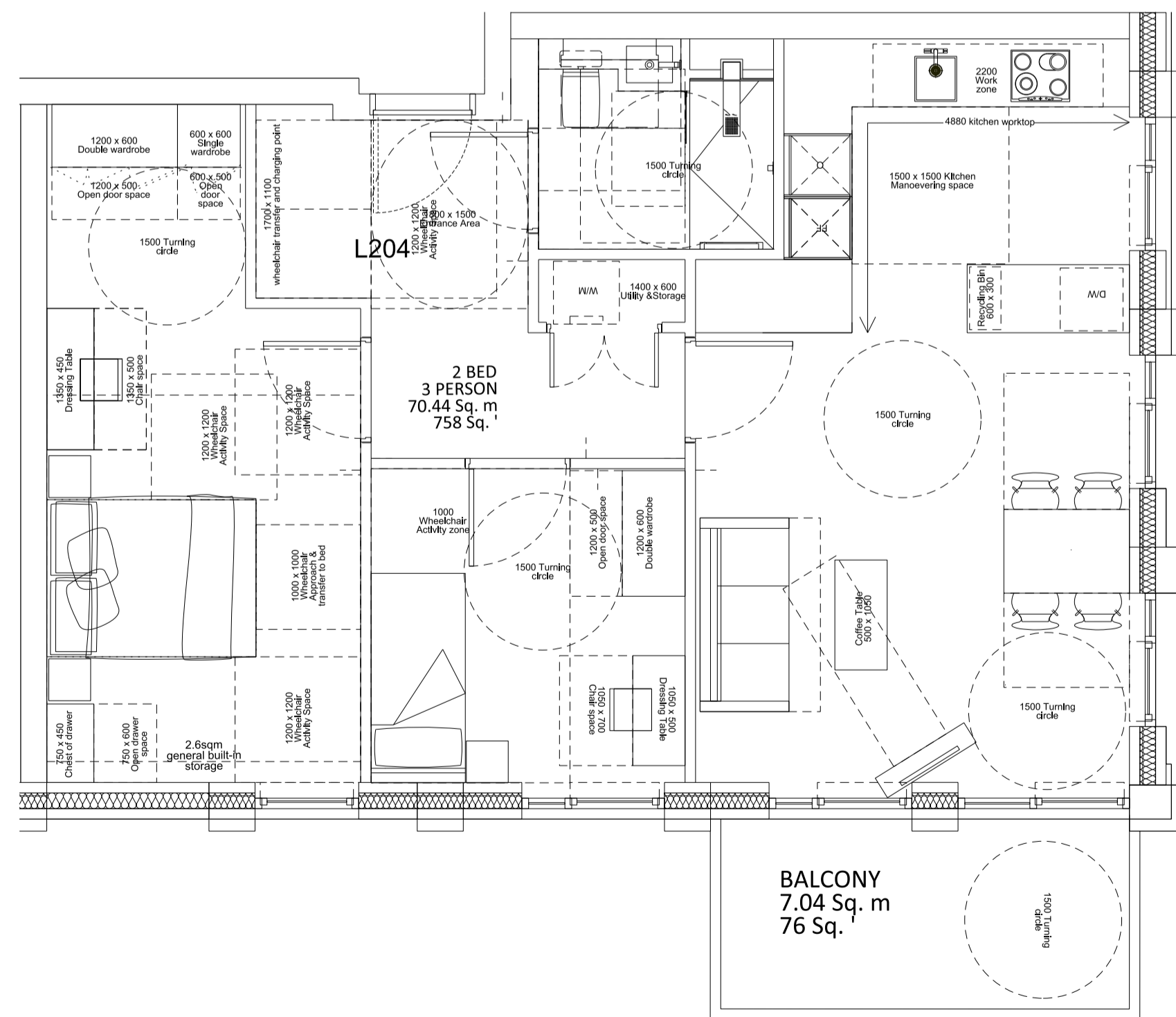
03 2 Bed Apartment M4(3)(2)(a)
