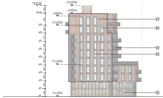
01 North Elevation Building C
