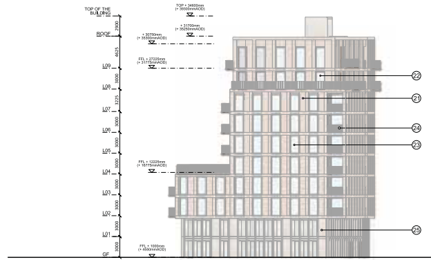
03 South Elevation Building C
