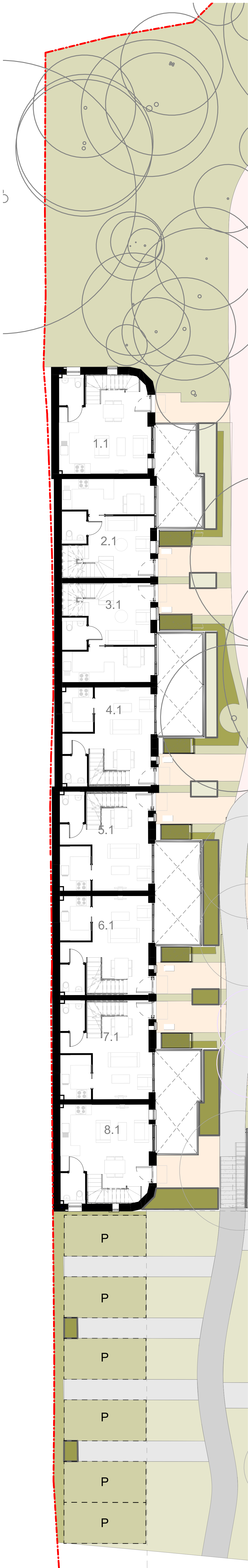
3 Block A - Plan GF 1 : 100
