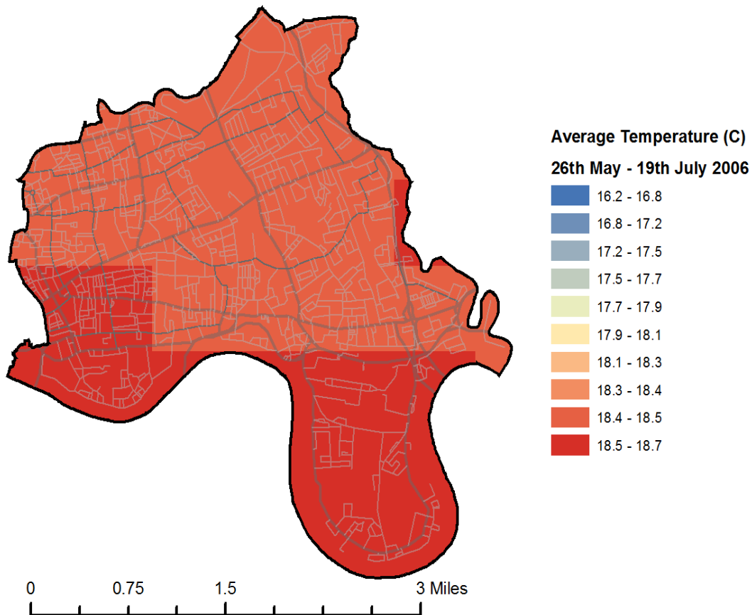
Figure 6: Average temperatures in Barnet
