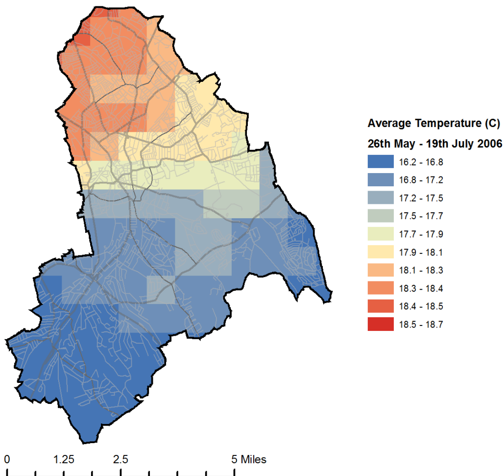
Figure 6: Average temperatures in Croydon
