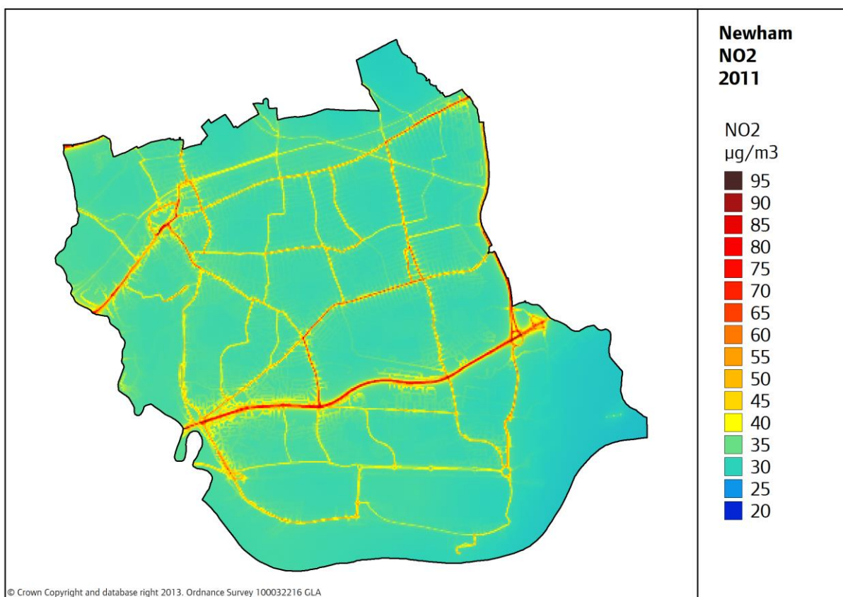
Figure 3 NO 2 emissions on Newham Roads
