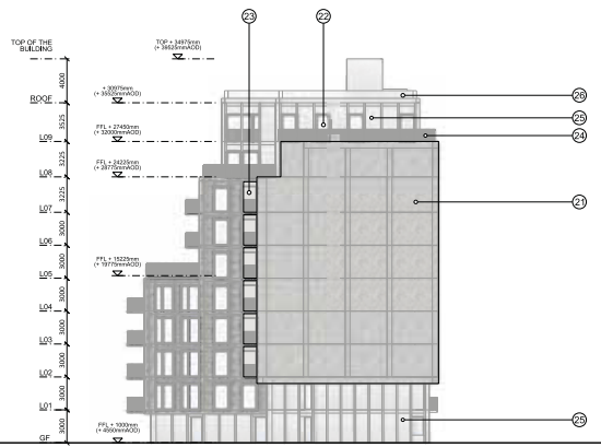
03 South Elevation Building A
