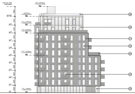
01 North Elevation Building A
