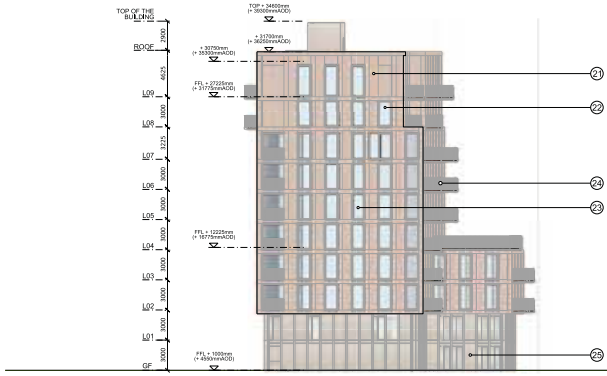
01 North Elevation Building C
