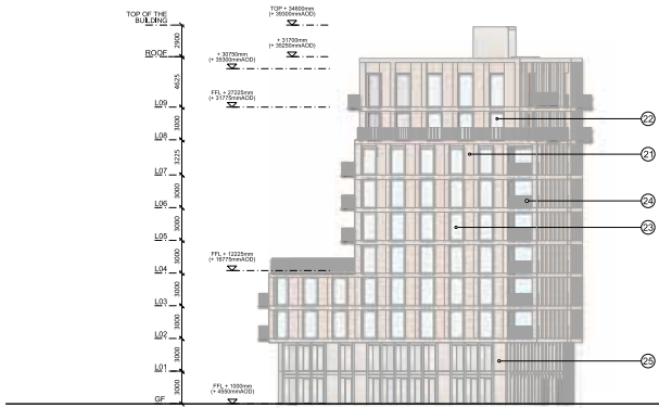
03 South Elevation Building C
