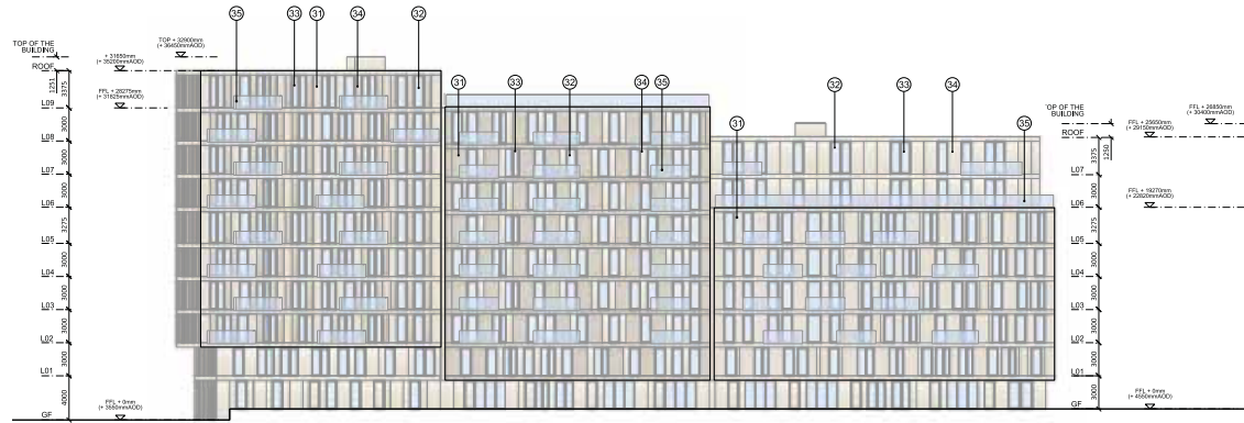
02 East Elevation Building EF
