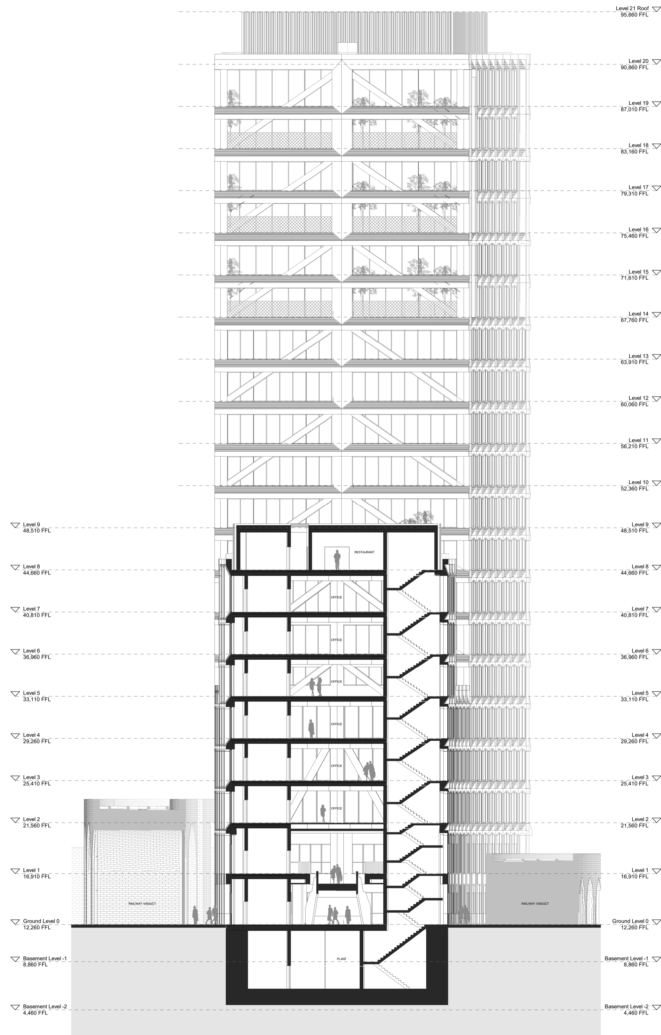
1 Proposed Cross Section E-E' 1:200
