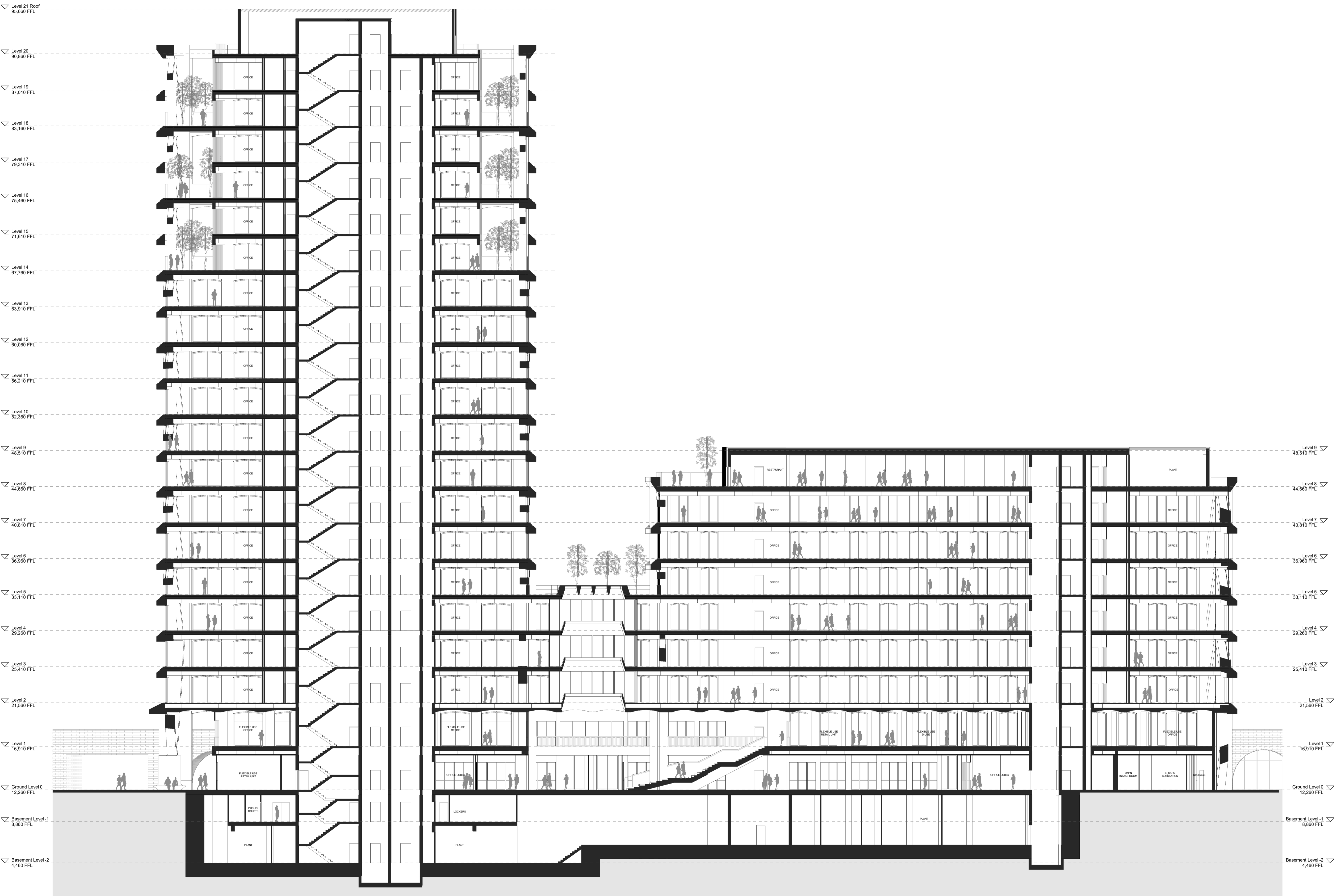
1 Proposed Longitudinal Section B-B' 1 : 200
