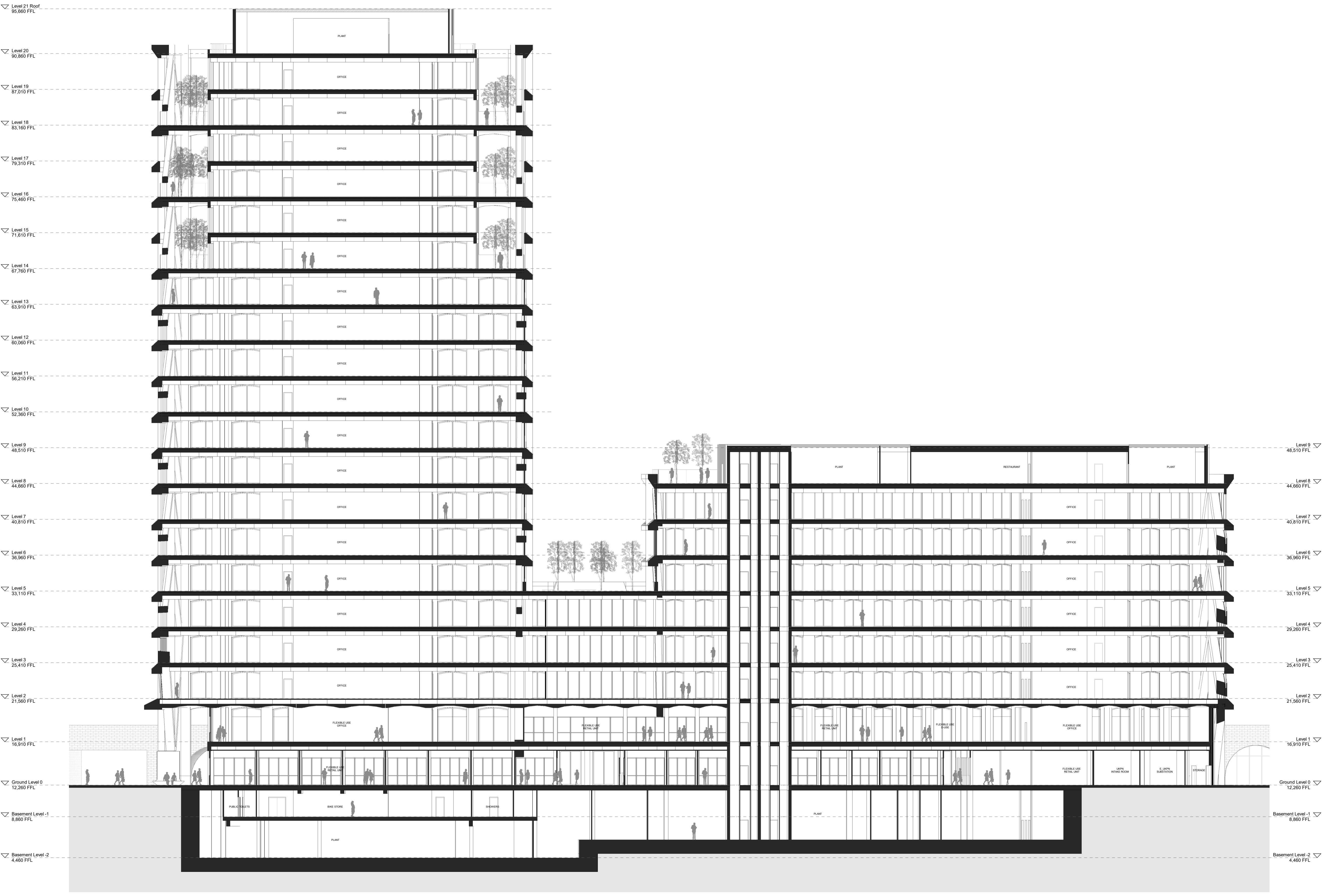
1 Proposed Longitudinal Section A-A' 1 : 200
