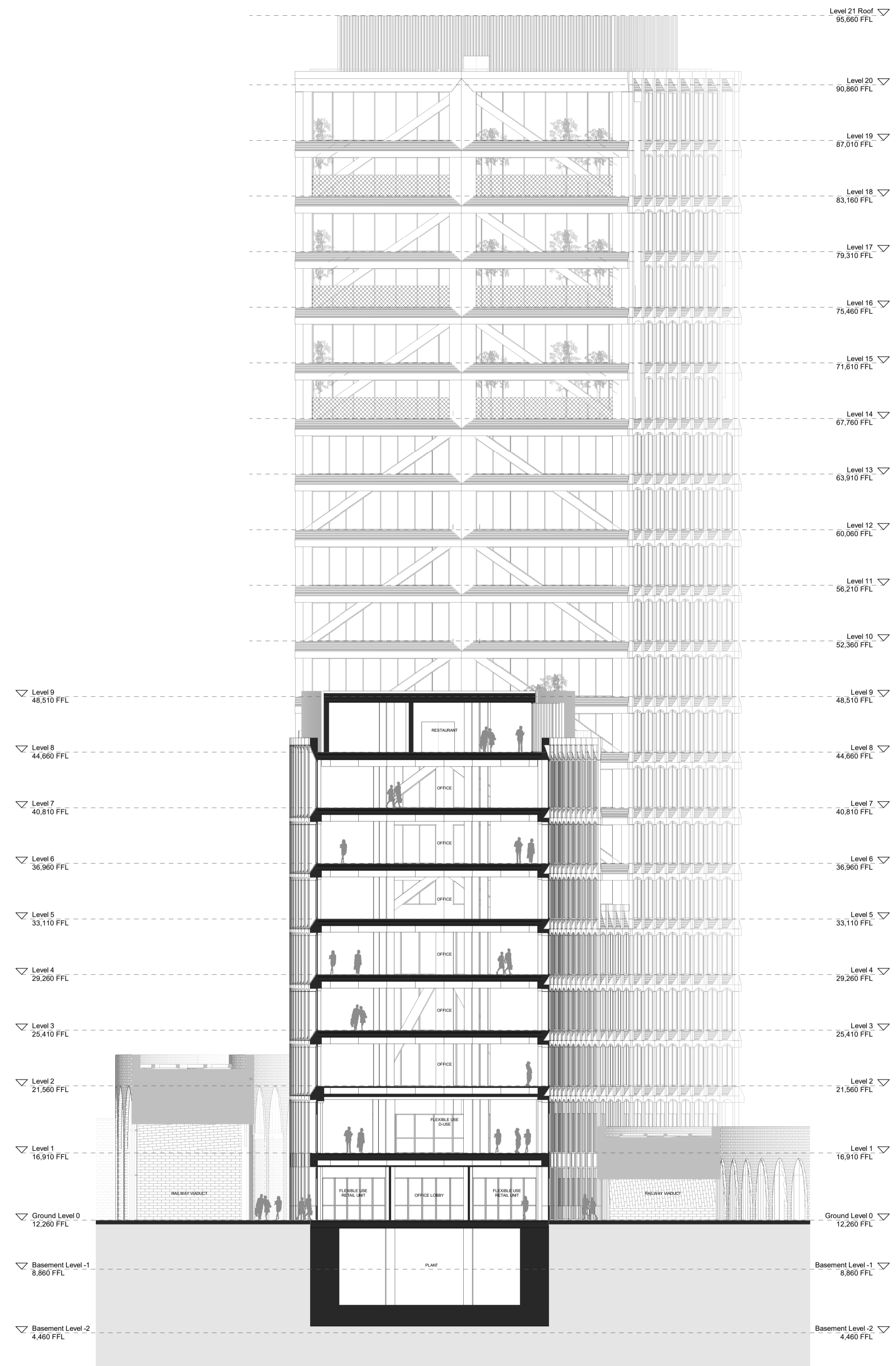
2 Proposed Cross Section F-F' 1:200
