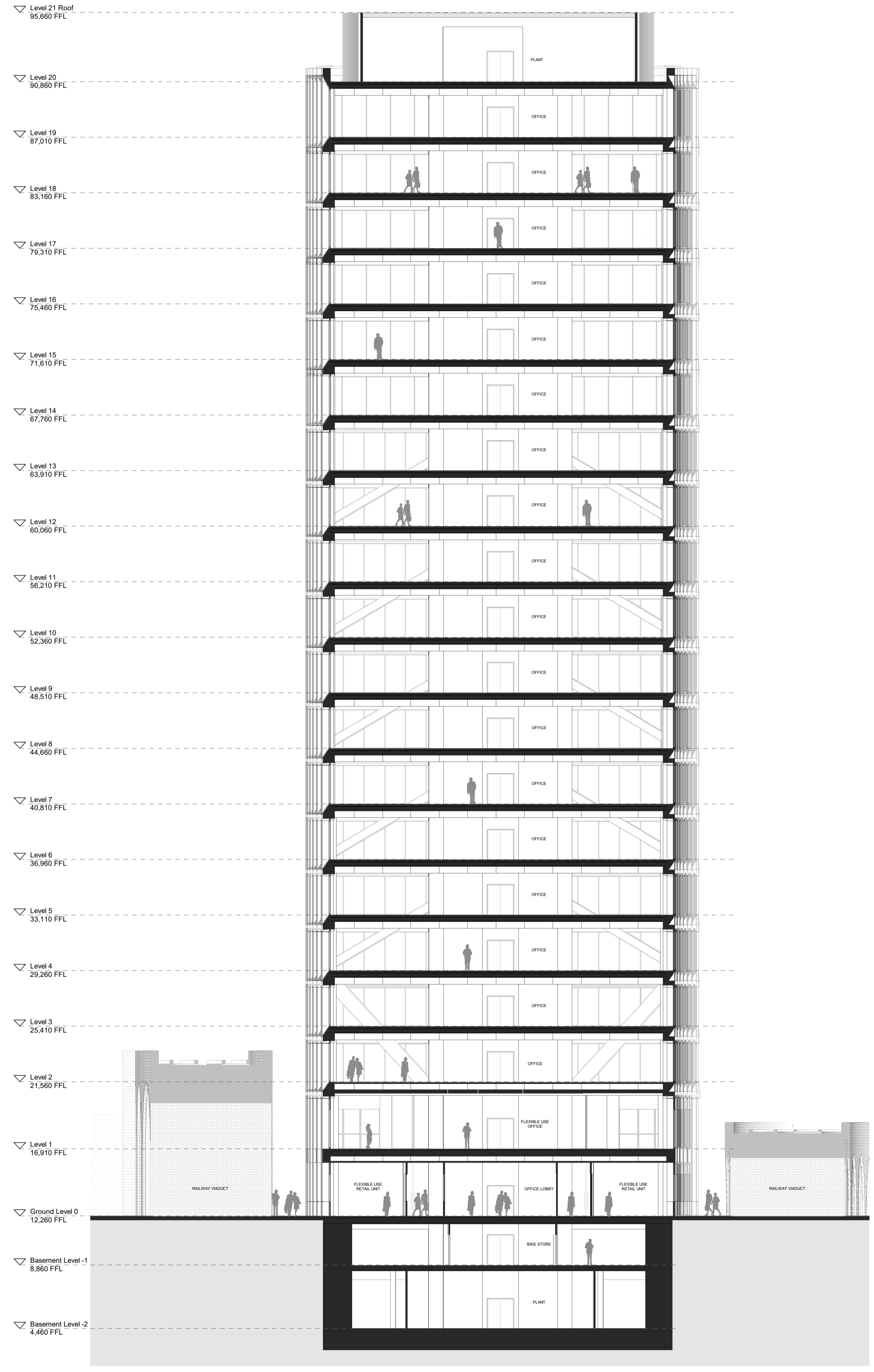
1 Proposed Cross Section C-C' 1 : 200
