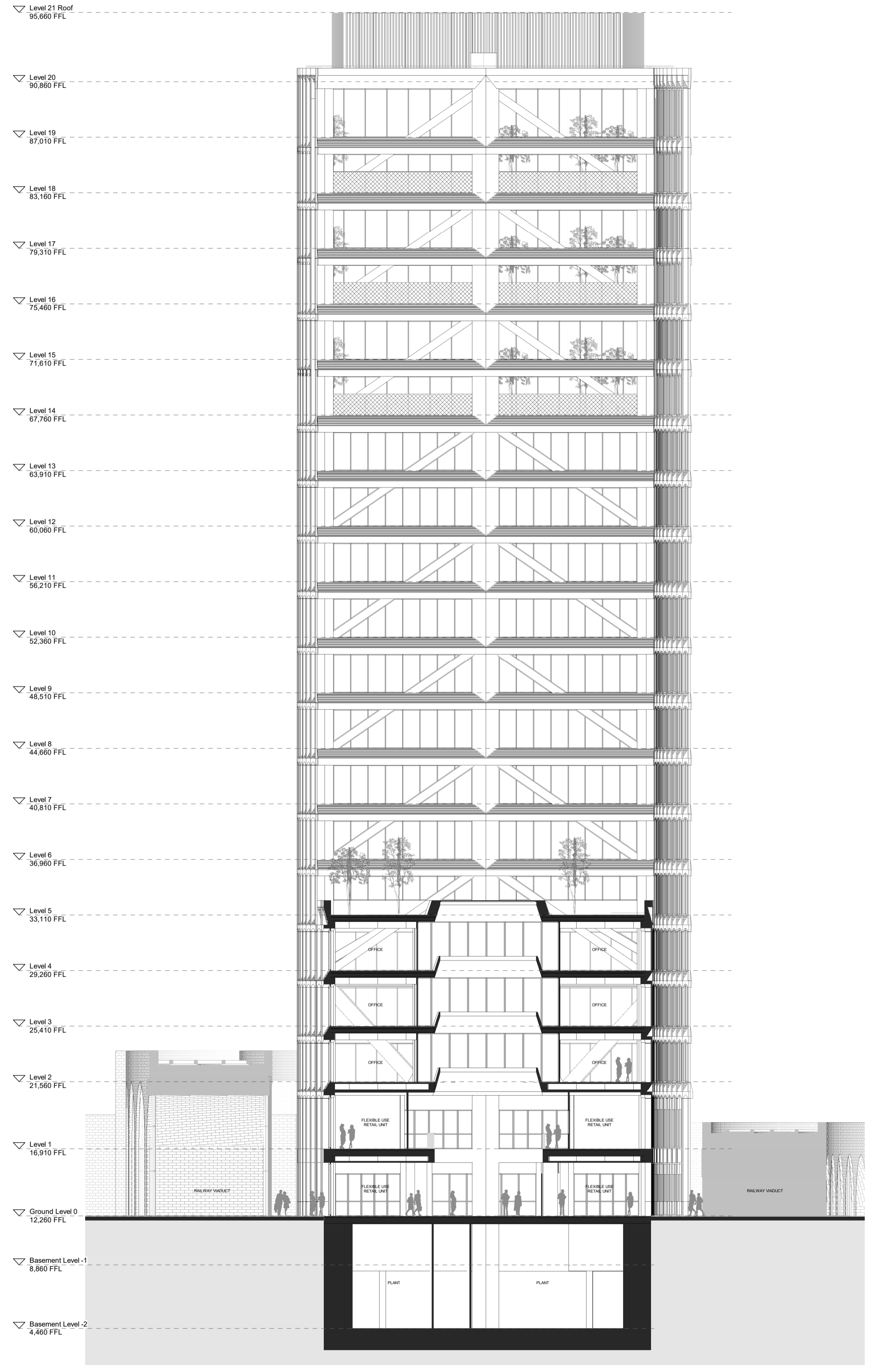
2 Proposed Cross Section D-D' 1 : 200
