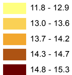
WSAVGMIN - average minimum daily temperature across the 2006 summer period (May 26th-August 31st)
